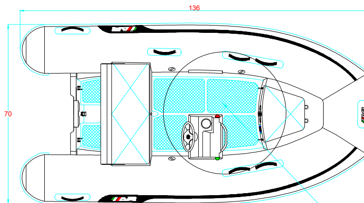
PLANT VIEW VISTA SUPERIOR
