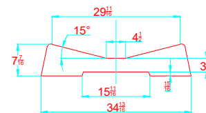
TRANSVERSAL SECTION "A" SECCION TRANSVERSAL "A"
